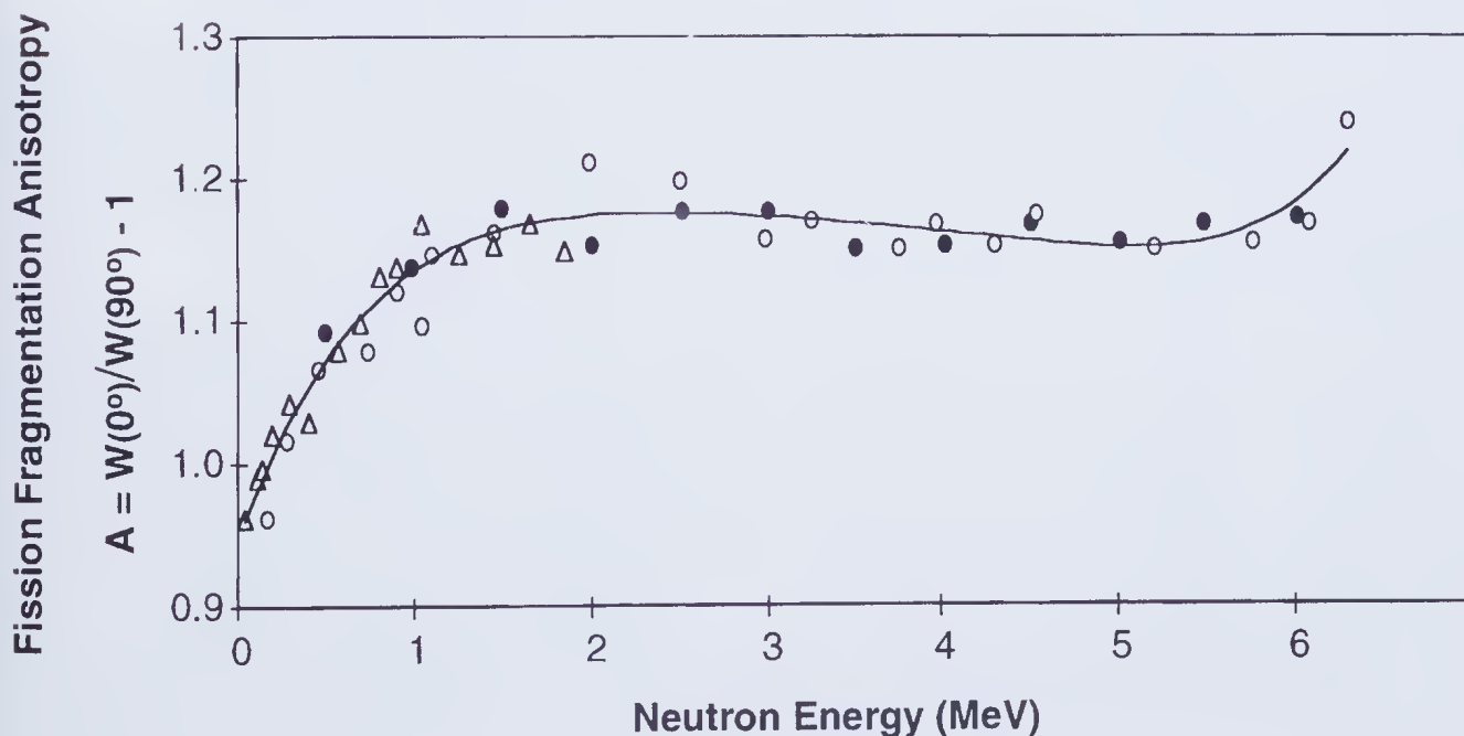
Figure 3. The ^{235}\text{U}(n,f) fission fragment anisotropy (modified from Straede et al. 1987).
